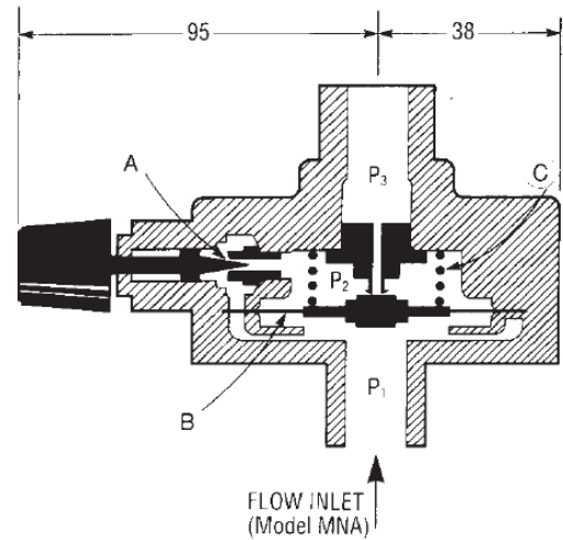
SECTION DIAGRAM
