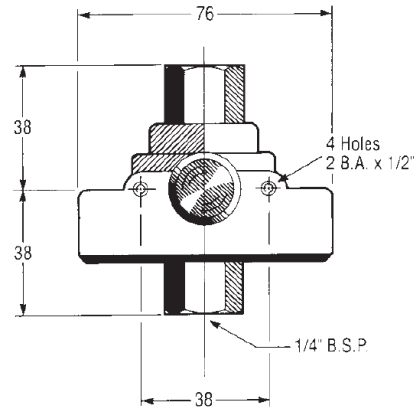
SECTION DIAGRAM
