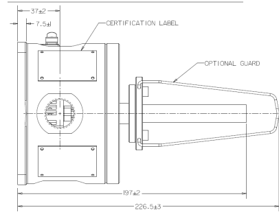
Ex d version
